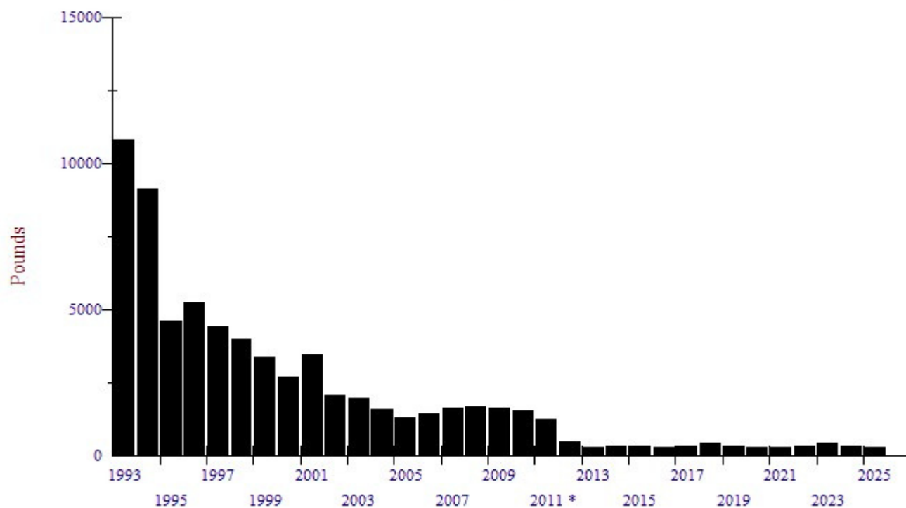
Field's Point Effluent Copper Loading
