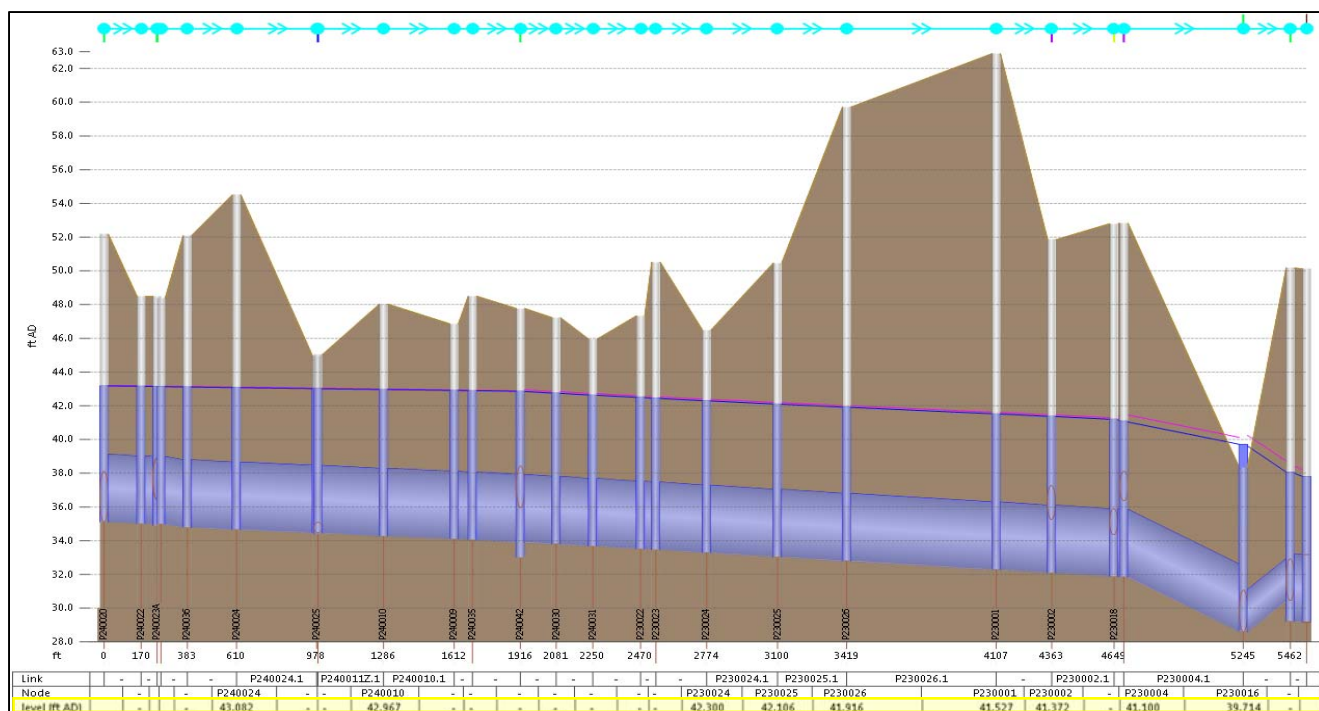
Figure 2.3. Upper BVI Profile Without Upper BVI Surcharge Relief-Peak 3-Month Storm
