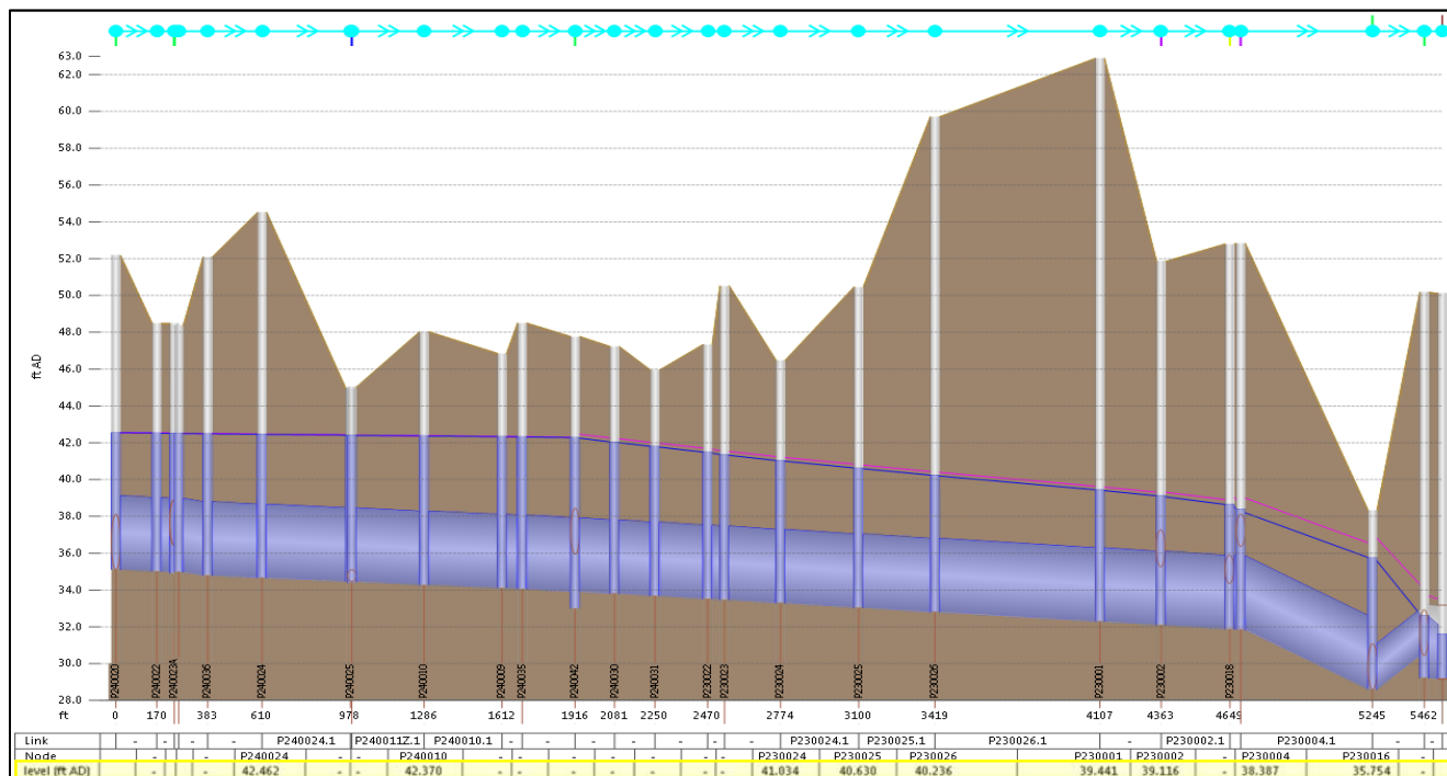
Figure 2.2. Upper BVI Profile-With Upper BVI Surcharge Relief-Peak 3-Month Storm
