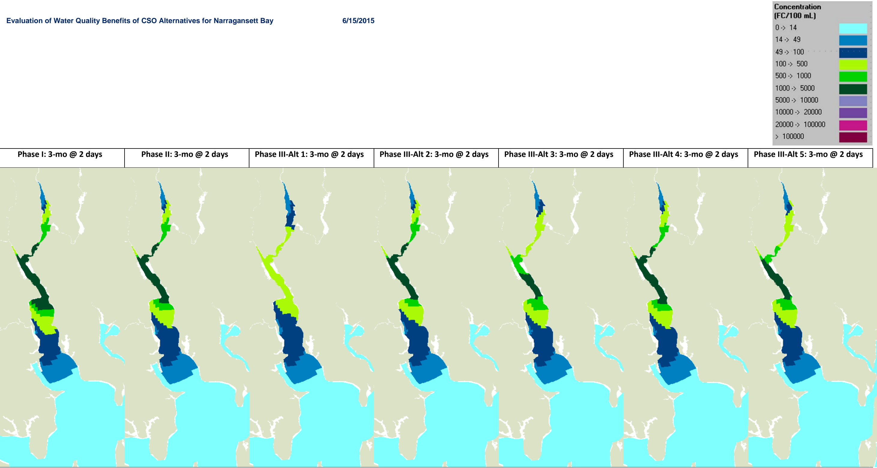
Figure 4-9. Scenario plan views of FC concentrations 2 days after start of 3-mo storm.
