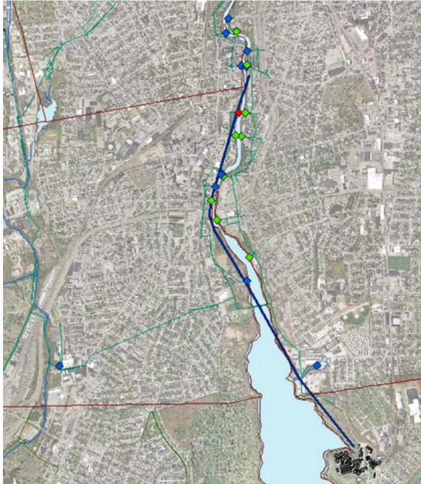
Figure 31 – Pawtucket Tunnel (CDRA Route)
