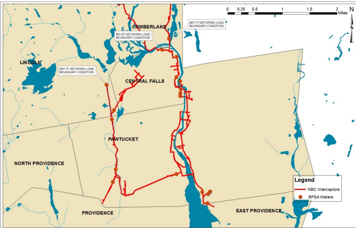
Figure 6: Bucklin Point Meters and Network Boundaries.
