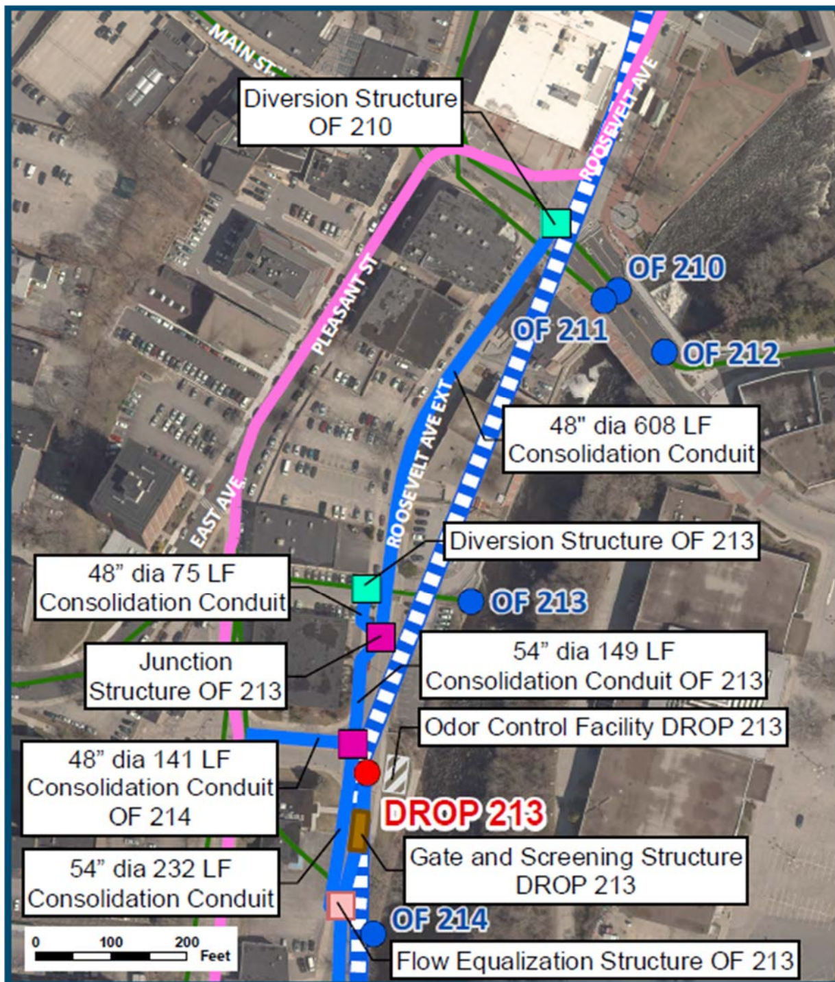
Figure 3.12. Alternative 3 Drop Shaft 213
